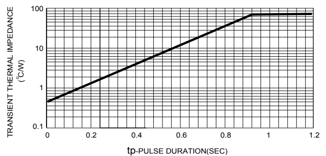
FIG.8- TYP. TRANSIENT THERMAL IMPEDANCE
